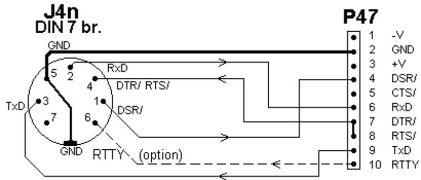
FIGURE 1 Câblage interne
